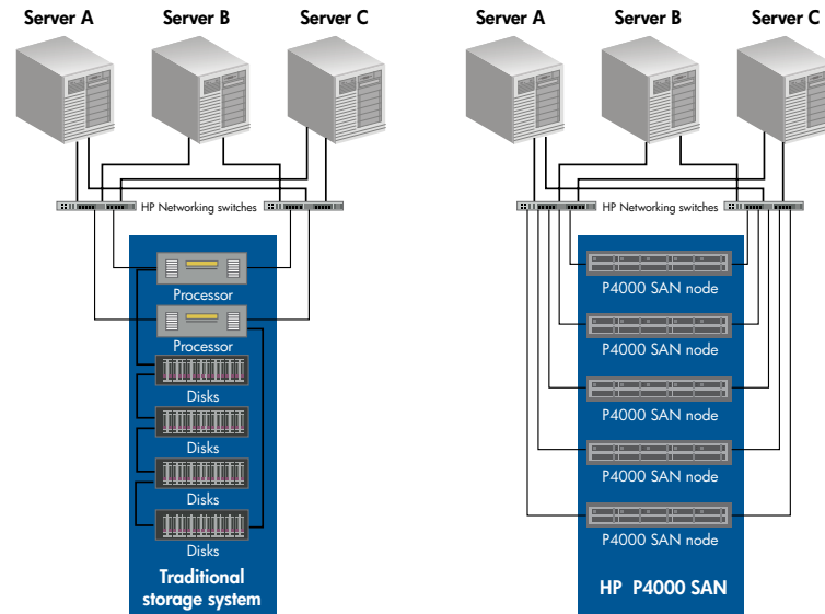
Figure 6: In contrast to traditional SANs whose performance is limited by fixed RAID groups and a centralized controller, HP P4000 SANs use storage clustering where every storage system contributes to the performance of every logical volume.
